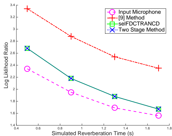
Fig. 6: Log Likelihood Ratio Results of Dereverberation Evaluation, selfDCTRANCD and Two Stage Method produce identical results.
