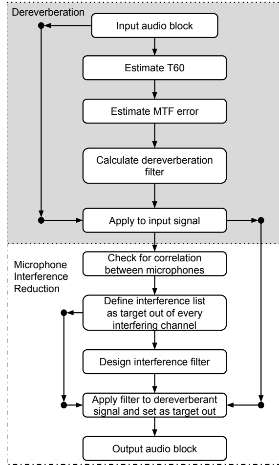
Fig. 2: Flow Diagram of the Two Stage Method
