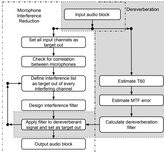
Fig. 3: Flow Diagram of selfDCTRANCD
