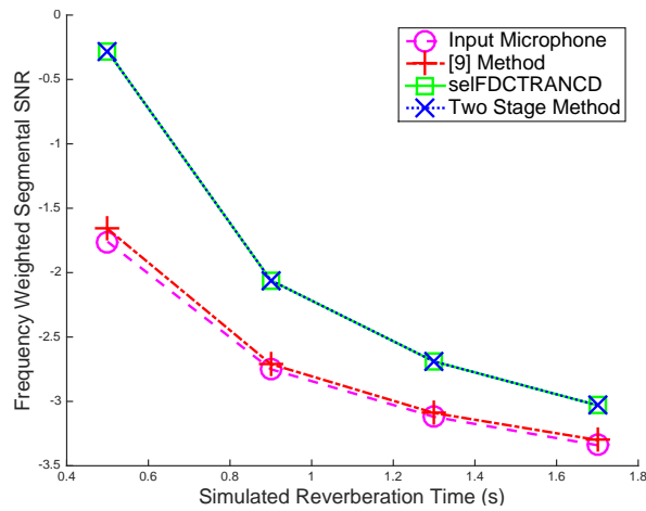
Fig. 8: Frequency-Weighted Segmental Signal to Noise Ratio Results of Dereverberation Evaluation, selfFDCTRANCD and Two Stage Method produce identical results.
