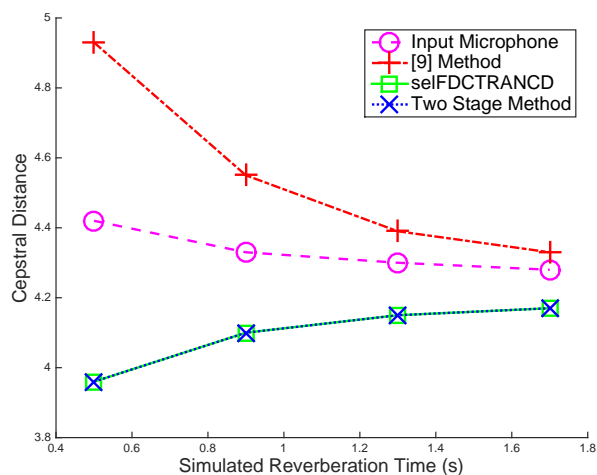
Fig. 5: Cepstral Distance Results of Dereverberation Evaluation, selfDCTRANCD and Two Stage Method produce identical results.
