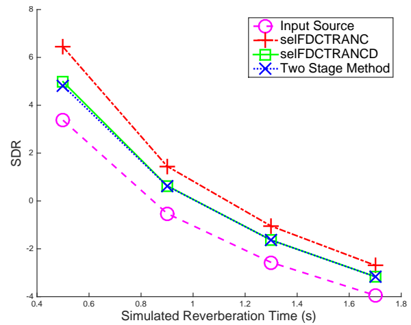
Fig. 9: Signal to Distortion Ratio Results of Microphone Interference Reduction Evaluation.
