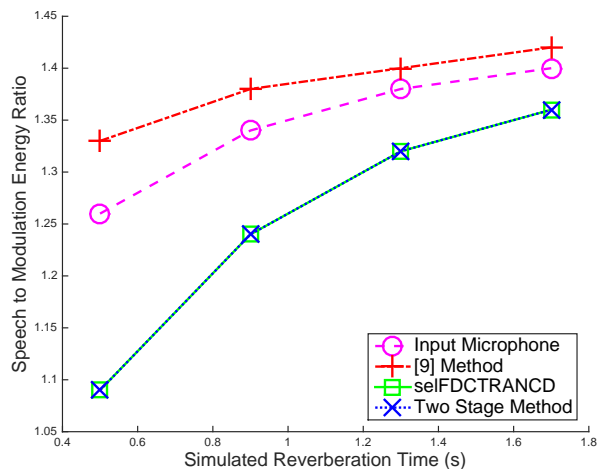
Fig. 7: Speech to Reverberation Modulation Energy Ratio Results of Dereverberation Evaluation, selfDCTRANCD and Two Stage Method produce identical results.
