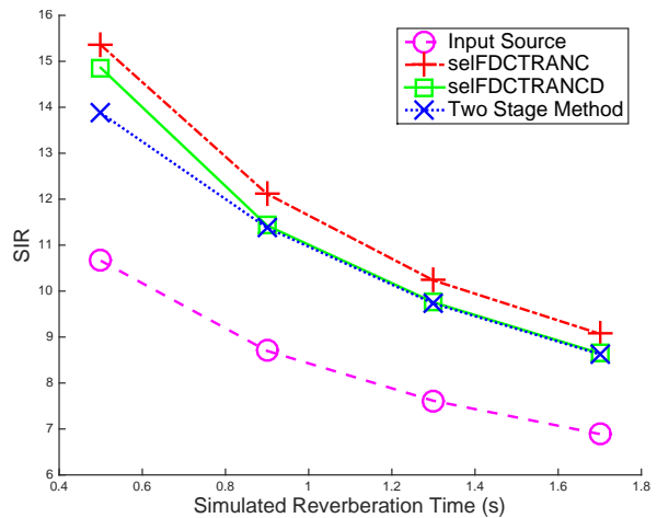
Fig. 10: Signal to Interference Ratio Results of Microphone Interference Reduction Evaluation.
