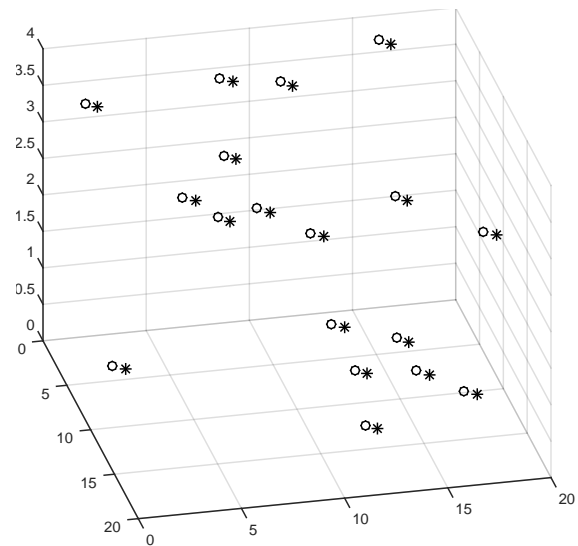
Fig. 4: Visualisation of Room Simulation. Room Size 20m x 20m x 4m. (o = Source, * = Microphone)
